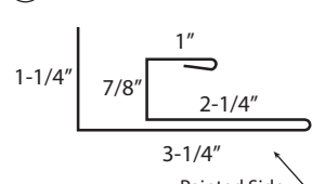
㉔ F & J Channel
