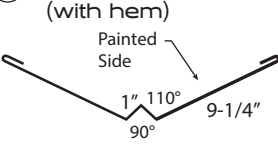
⑯ "W" Valley* (with hem)
