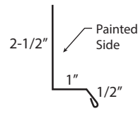
㉑ Base Trim
