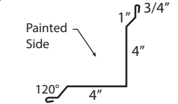
⑮ Inside Corner
