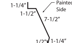
⑬ 2-1/2" Outside Corner*
