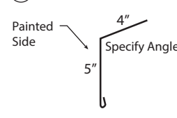
⑫ 4" Outside Corner*
