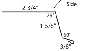
㉓ Double Angle
