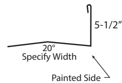
⑧ Eave Trim/Upper Gambrel
