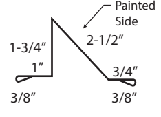
㉕ Chimney Counter Flashing
